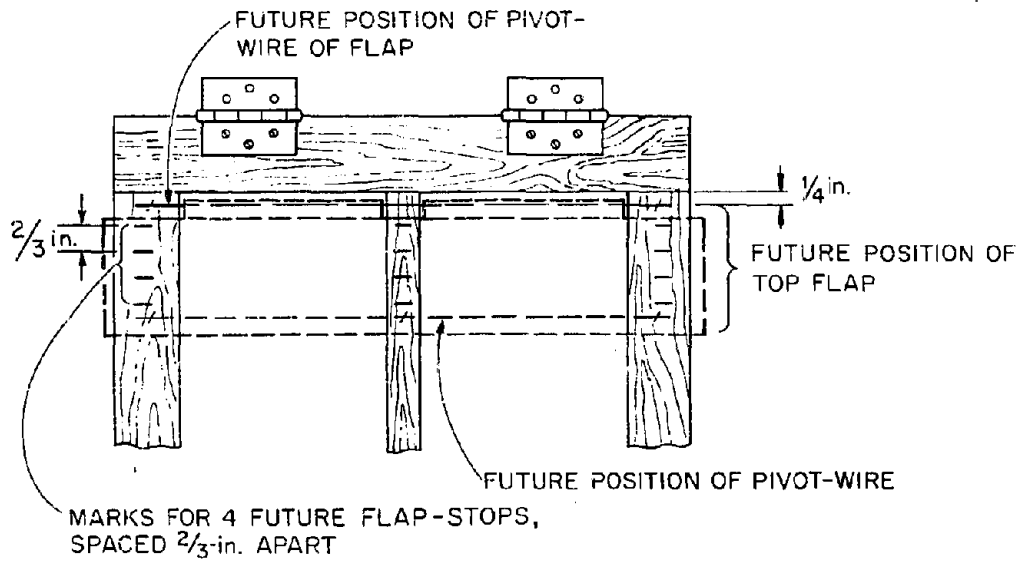
Fig. B-10. Marking for flap stops.
